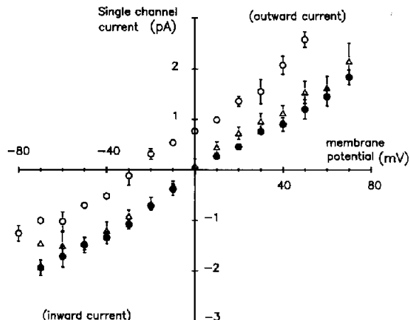
Fig.3. Single-channel current as a function of vacuolar membrane potential in tomato. The I - V relationship of tonoplast patches exposed to symmetrical solutions of 100 mM KCl ( \bullet ) was linear between -80 mV and 80 mV, with a conductance of 29 pS, with a reversal potential of 0 mV. Establishing a K^+ concentration gradient across the patch ( 100 mM K^+ / 10 mM K^+ ) ( \circ ), shifted the zero membrane current to a potential of -30 mV. The conductance of the channel however, was not altered by the reduction of external KCl. Substitution of Na^+ for K^+ ( 100 mM K^+ / 100 mM Na^+ ) ( \Delta ), yielded a linear I - V relationship with a reversal potential of 0 mV and a conductance of 29 pS. Pipette and bath solutions always contained 2 mM MgCl_2 , 0.1 mM CaCl_2 , 5 mM Tris-Mes, pH 7.5 , and adjusted to an osmolarity of 550 mOsmol with mannitol. Points are the mean \pm SE ( n = 8 ).
