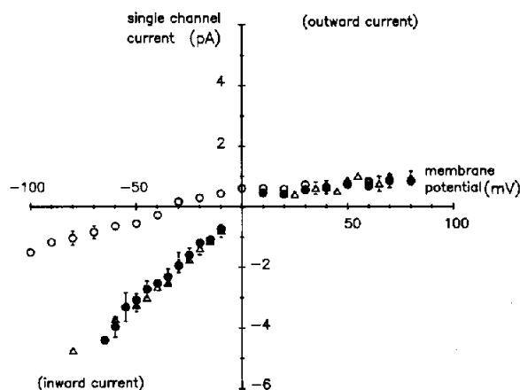
Fig.2. Single-channel current as a function of vacuolar membrane potential in sugar beet. Under symmetrical 100 mM KCl ( \bullet ), the I - V relationship is linear between -80 mV and 0 mV, with a reversal potential of 0 mV, and the slope giving a conductance of 65 pS. At pipette positive potentials, the conductance decreased to 10 pS. With 100 mM KCl in the pipette and 10 mM KCl in the bath ( \circ ), the reversal potential shifted towards a negative potential of -40 mV (average value). The conductance under asymmetrical K^+ concentrations, decreased to 20 pS. Substitution of 100 mM Na^+ for 100 mM K^+ in the bath ( \Delta ) did not change either the conductance of the channel, or its reversal potential. In addition to the different concentrations of K^+ and Na^+ , pipette and bath solutions also contained 2 mM MgCl_2 , 0.1 mM CaCl_2 , 5 mM Tris-Mes, pH 7.5 , and mannitol to give a final osmolarity of 550 mOsmol. Points are the mean \pm SE ( n = 8 ).
