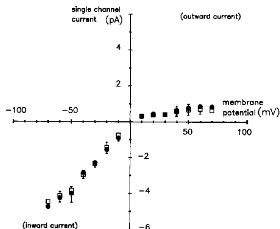
Fig.4. Effect of DIDS on the inward rectifying currents of sugar beet tonoplast. The voltage-dependence of the single-channel currents of sugar beet tonoplast patches, exposed to symmetrical KCl ( \bullet ), was not altered by the addition of 100 \mu M DIDS ( \square ). The data for the DIDS experiments are the mean \pm SE ( n = 4 ).
